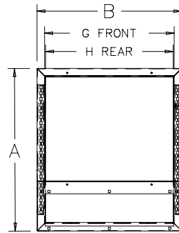
600 mm wide Sloped Top with Accessory Front
